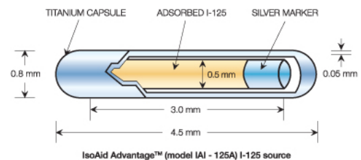
IsoAid Advantage™ (model IAI - 125A) I-125 source
