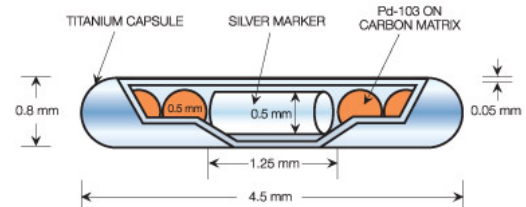
IsoAid Advantage™ (model IAPd - 103A) Pd-103 source
